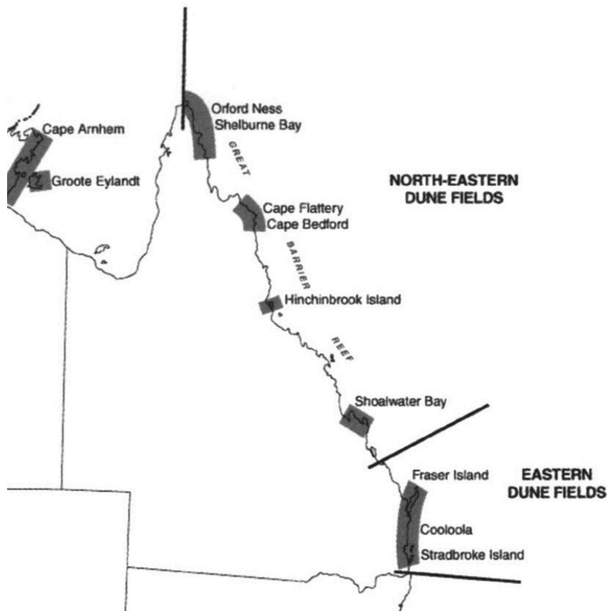
Figure 8 Location of major coastal dune fields in northern and eastern Australia (Lees 2006)
