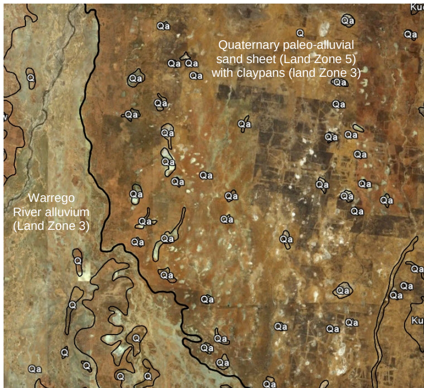
Plate 20 Image of paleo-sandy alluvium of Land Zone 5
