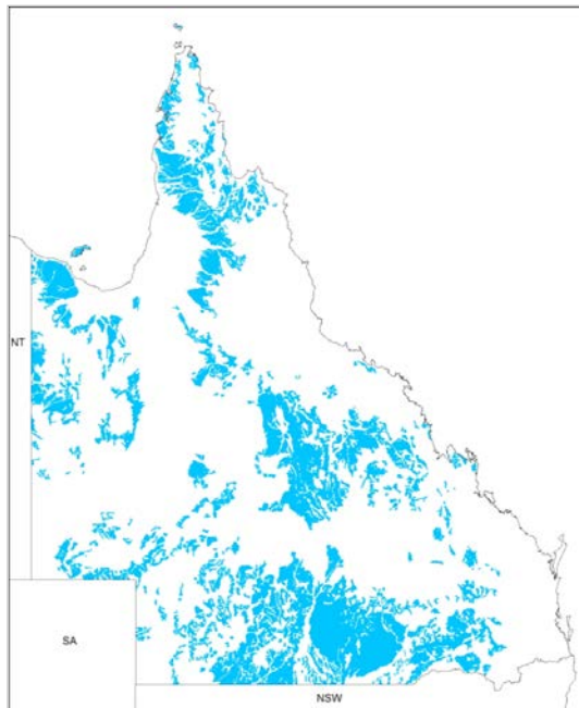
Figure 11 Late Cainozoic floodout and residual sand, soil and gravel
