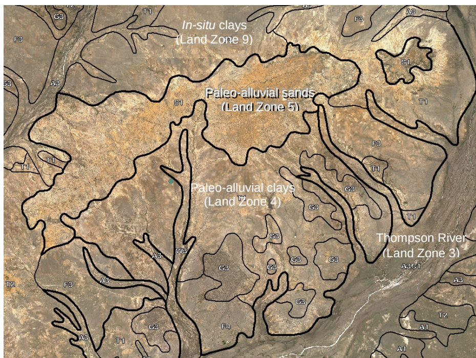
Plate 21 Elevated Tertiary sand alluvia (S1) associated with a paleo-river system not associated with the current Thompson River
