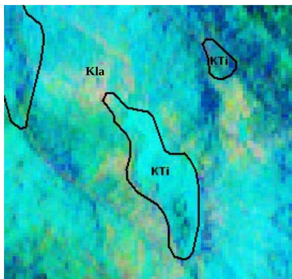
Plate 23 Geology and radiometrics (K, Th and U radioisotope signature of earth's surface) of Batavia Downs, Cape York Peninsula.
