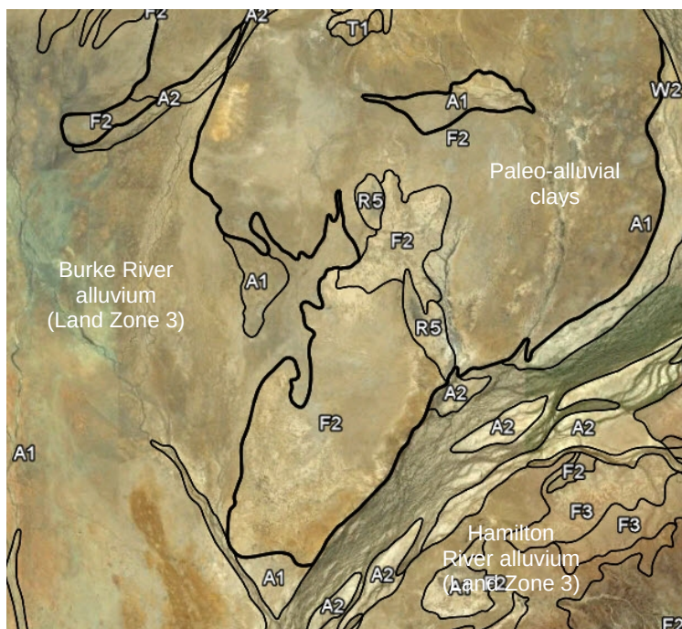
Plate 15 Paleo alluvial clay plains (F2) of Land Zone 4
