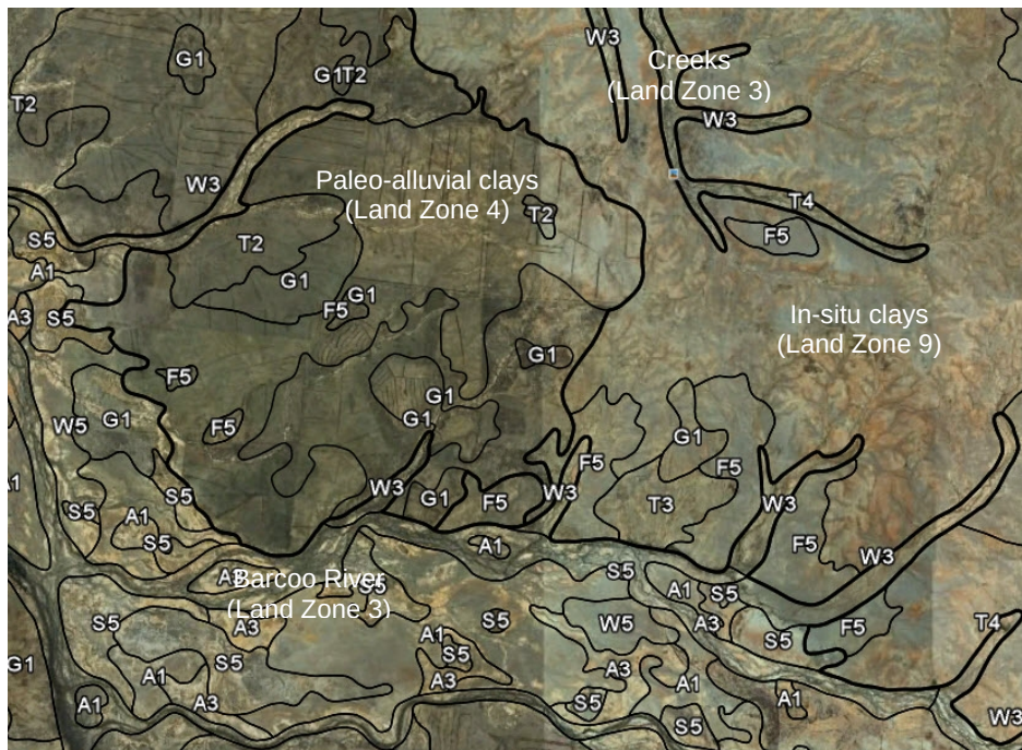
Plate 14 Paleo-alluvial clay soils of Land Zone 4 associated with gidgee (G1, T2)
