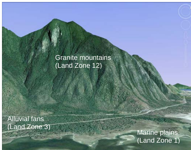
Plate 13 Quaternary alluvial fans of Mt Elliott, south of Townsville with streams and gullies from Mt Elliott aggrading fans onto the coastal marine plains (Google Earth)
