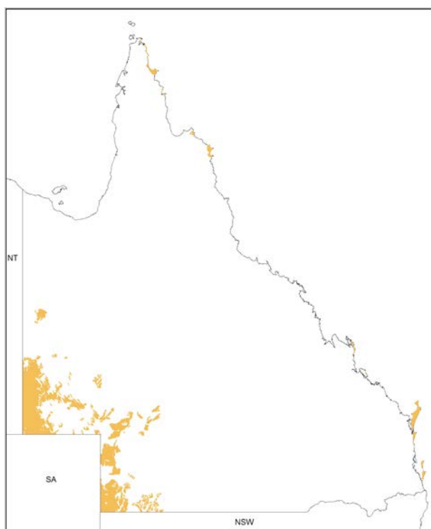
Figure 13 Location of major coastal (Land Zone 2) and inland (Land Zone 6) dunefields
