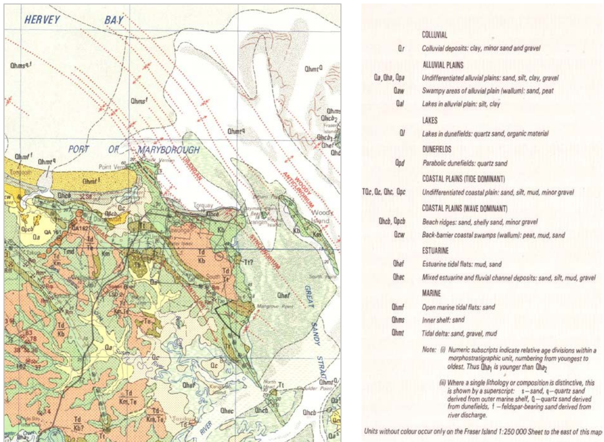
Figure 1 Geology mapping of Hervey Bay with numerous subdivisions of tidal and sub-tidal sediments (1:250 000 geology map)
