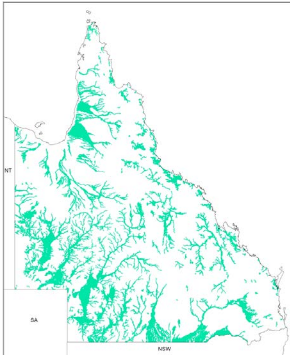
Figure 10 Major Quaternary alluvial deposits (Queensland Geology 1:2 500 000)
