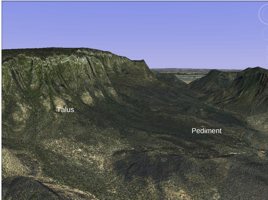
Plate 33 Sandstone cliffs, talus and sandy pediments of the Blackdown Tablelands are all Land Zone 10 (Google Earth)
