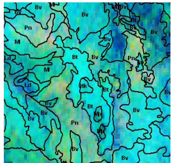
Plate 24 Picanninny (Pn) and Myall (M) clay soils developed in-situ on labile sediments of the Rolling Downs Group (KLa) (Land Zone 9) both have high K radiometrics.
