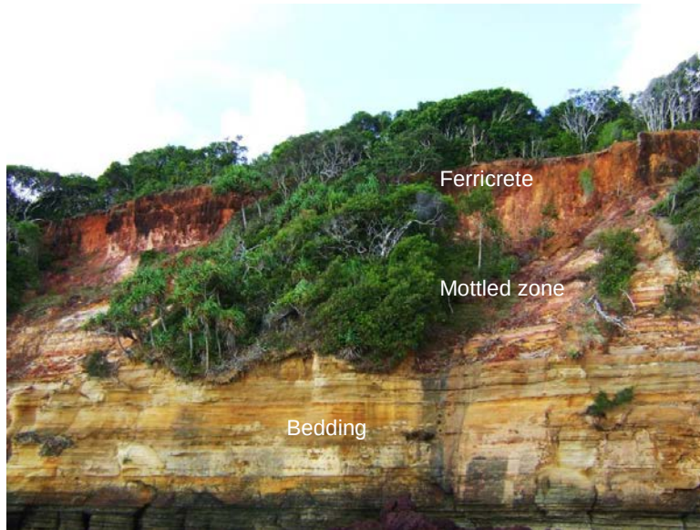
Plate 31 Deeply weathered Helby Beds (Land Zone 5) on Cape York Peninsula
