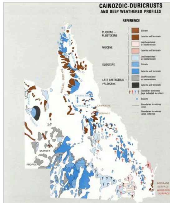
Figure 12 Cainozoic duricrusts and deeply weathered profile (Day et al. 1983)
