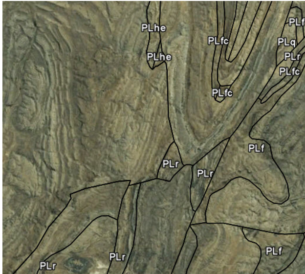
Plate 34 Strongly folded and strongly metamorphosed geologies (Land Zone 11) of the Mt Isa Inlier (Google Earth)
