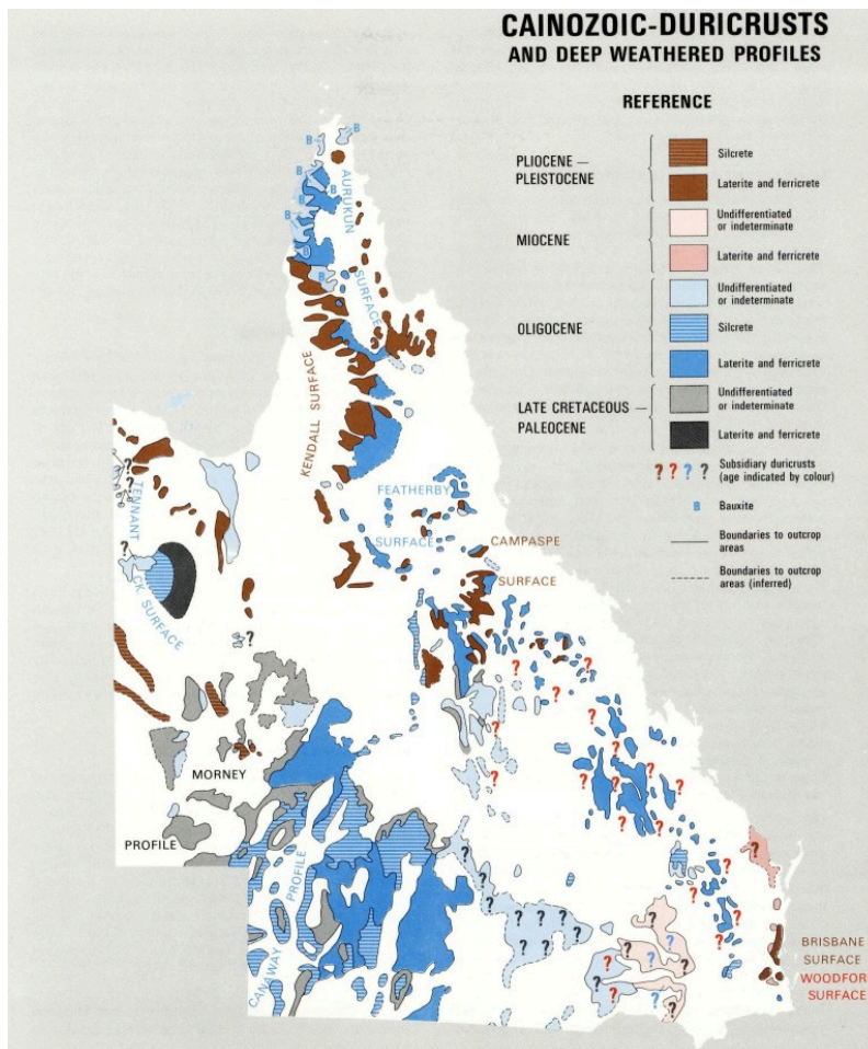
Figure 3 Cainozoic duricrusts and deep weathering profiles in Queensland (Day et al. 1983)
