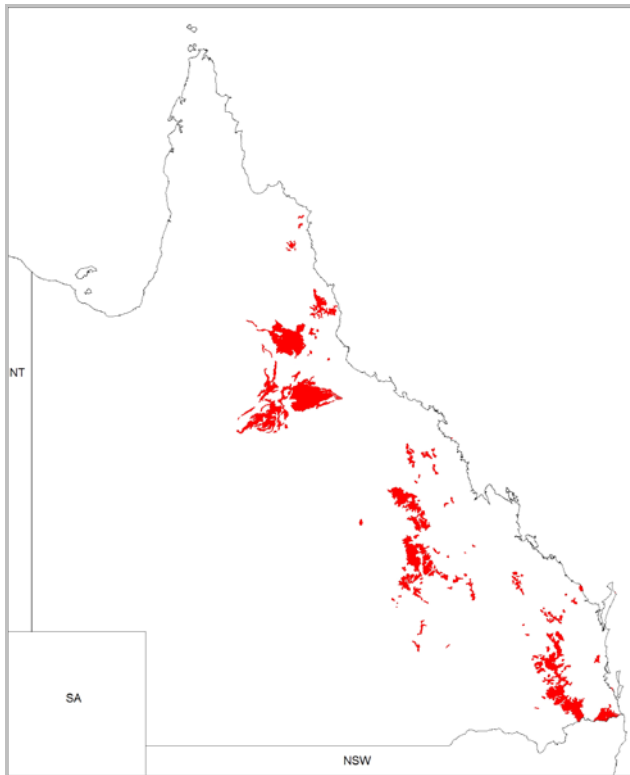
Figure 14 Location of Cainozoic igneous rocks
