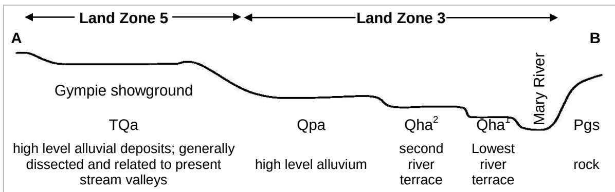
Figure 9 Cross-section (A-B) across the Mary River to Gympie showground (see Plate 42)
