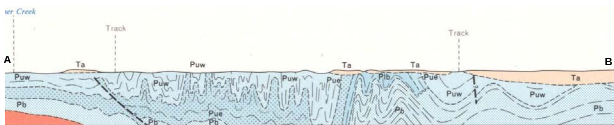
Figure 6 Cross section (A–B) showing strongly folded sediments of Blackwater Group (Puw) (1:250 000 geology map)
