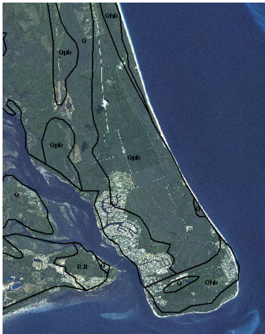
Plate 7 Pleistocene and Holocene beach ridges on Bribie Island (Google Earth)
