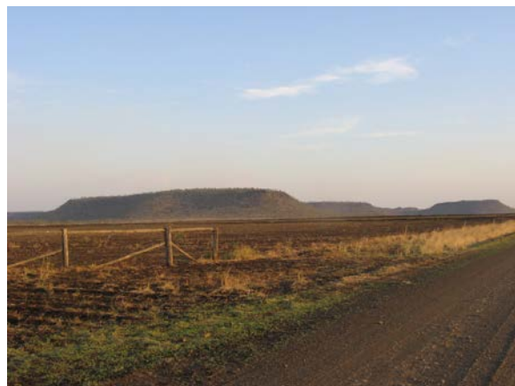
Plate 57 Tertiary basalt plateau remnants and gently undulating plain, Minerva Hills, north of Springsure
