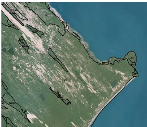
Plate 9 Longitudinal dunes of Cape Flattery (Google Earth)
