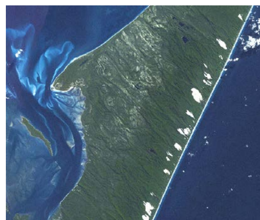
Plate 10 Longitudinal dunes of Fraser Island (Google Earth)
