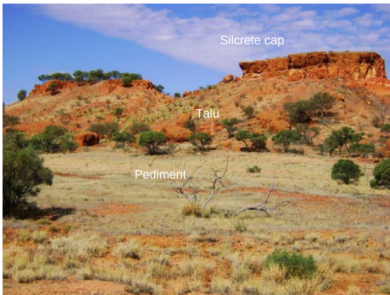
Plate 30 Duricrusted deeply weathered Winton Formation (Land Zone 7), west of Winton
