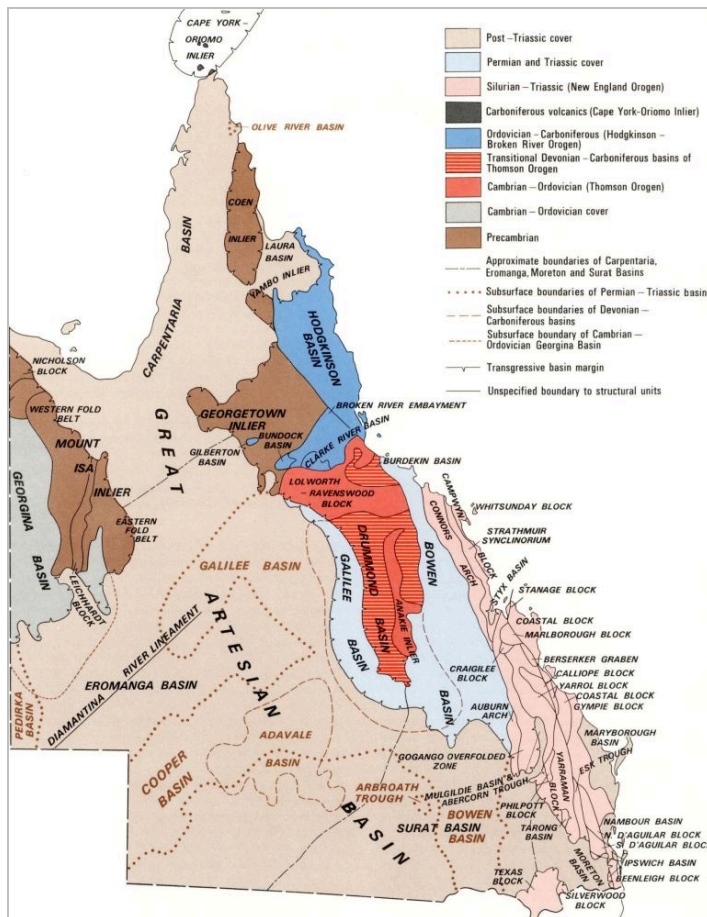
Figure 7 Geological structural framework (1: 2 500 000 Queensland Geology, Day et al. 1983)
