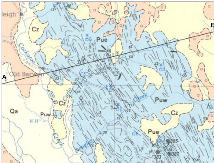
Figure 5 1:250 000 geology map of the same area as Plate 35 showing surface strike, dip and trend lines
