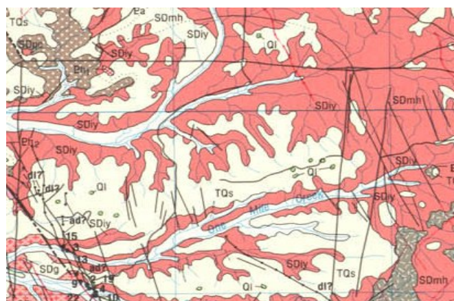
Figure 2 Deep transported sands (TQs) overlying granite (SDly) and other geologies
