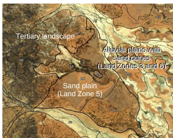
Plate 48 Sheet wash sand plains (Land Zone 5) southwest of Windorah developed from the erosion of the Tertiary landscape (western side of image) (Google Earth)
